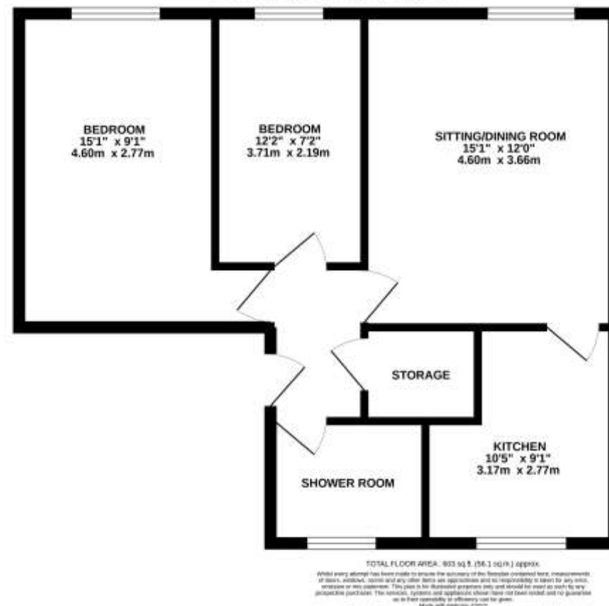
GROUND FLOOR 603 sq.ft. (56.1 sq.m.) approx.
